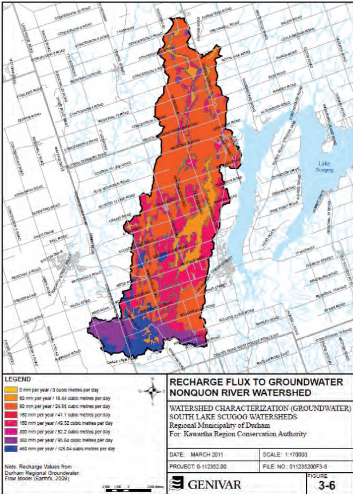
Figure 6.14: Recharge flux to groundwater.
