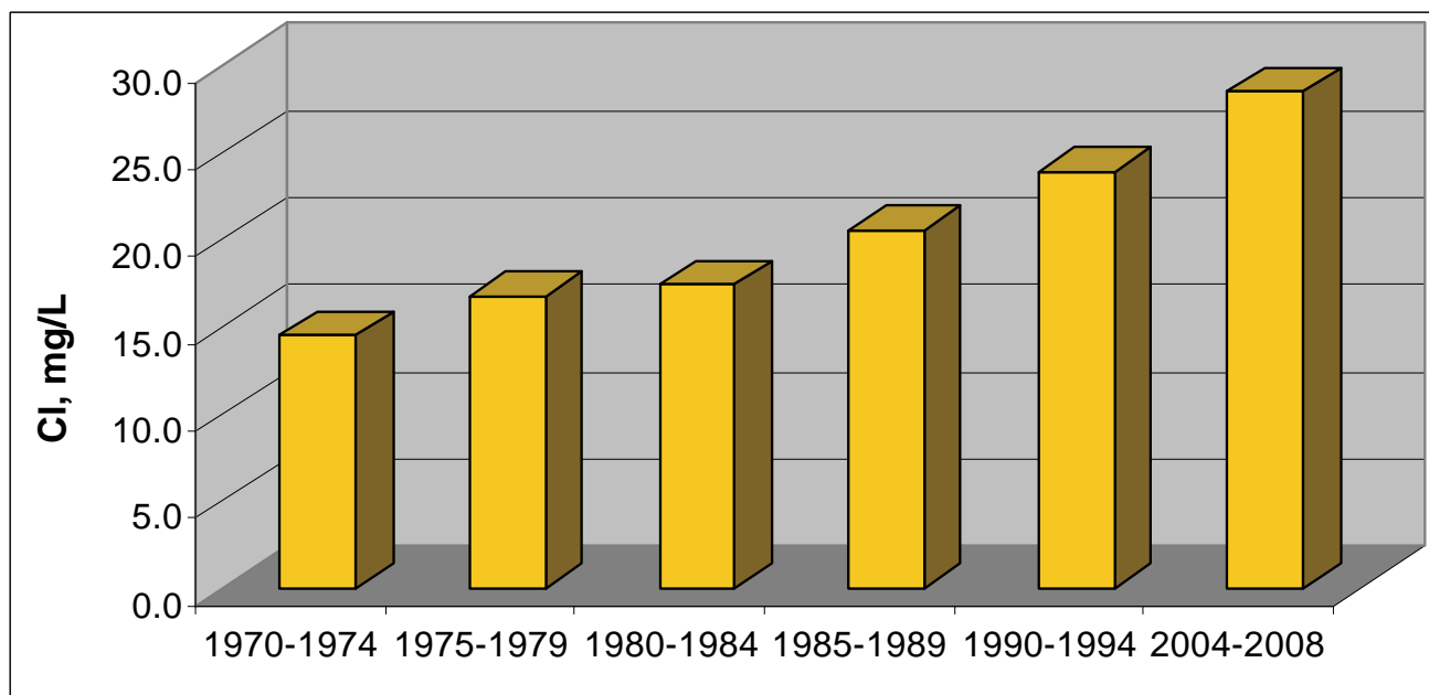
Figure 7.8: Long-term average Chloride concentrations in the Nonquon River near Seagrave during 1970 – 2008 monitoring period.
